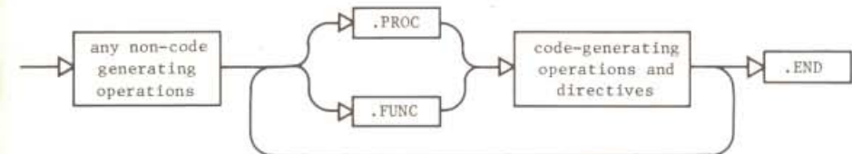
ASSEMBLY-FILE SYNTAX
