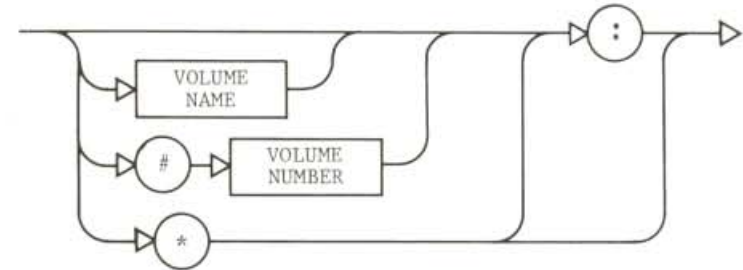
VOLUME-SPECIFICATION SYNTAX
